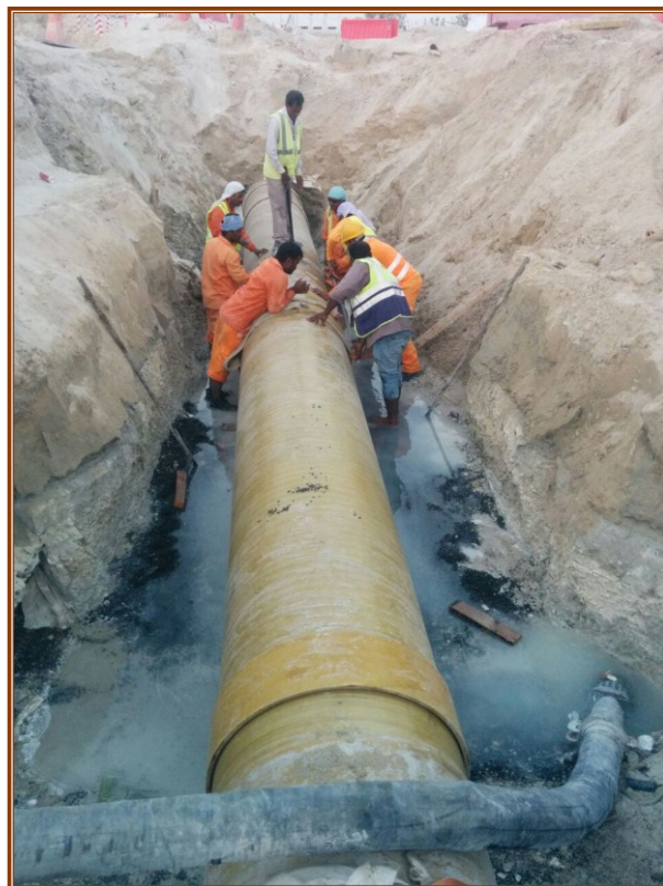
DIA900mm PIPE SHUTDOWN WORK AT DUBAI DESIGN DISTRICT
